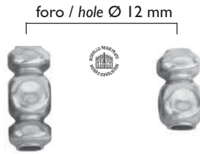
Art. 742/3 H 65 mm 25 x 25 mm sp/thick 2 mm
