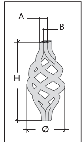
Art. 1163/9 Ø 70 mm B = Ø 6 mm
